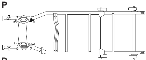
UNDERBODY VIEW
